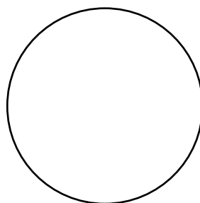
Full Moon
