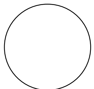
Waxing Gibbous
