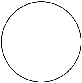
New Moon
